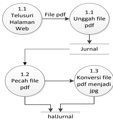
Gambar 4. Data Flow Diagram Rinci Proses 1
